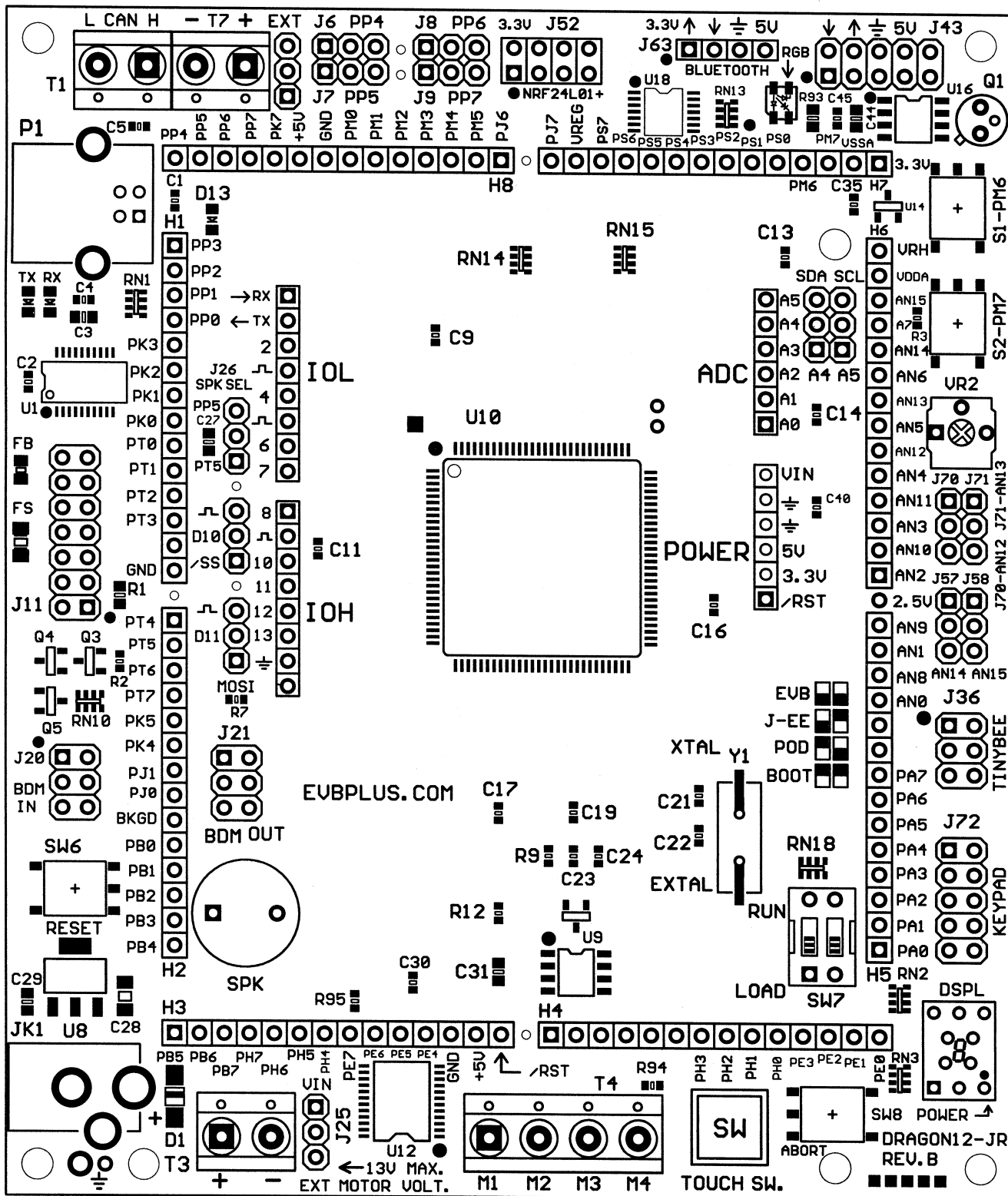
DRAGON12-JR REV B.
